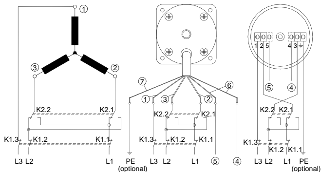
Figure 3: Three-phase motor: proposed circuit layout for switching on/off and reversing with mechanical contacts
